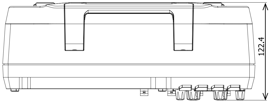
Figure 1-2 Top View
